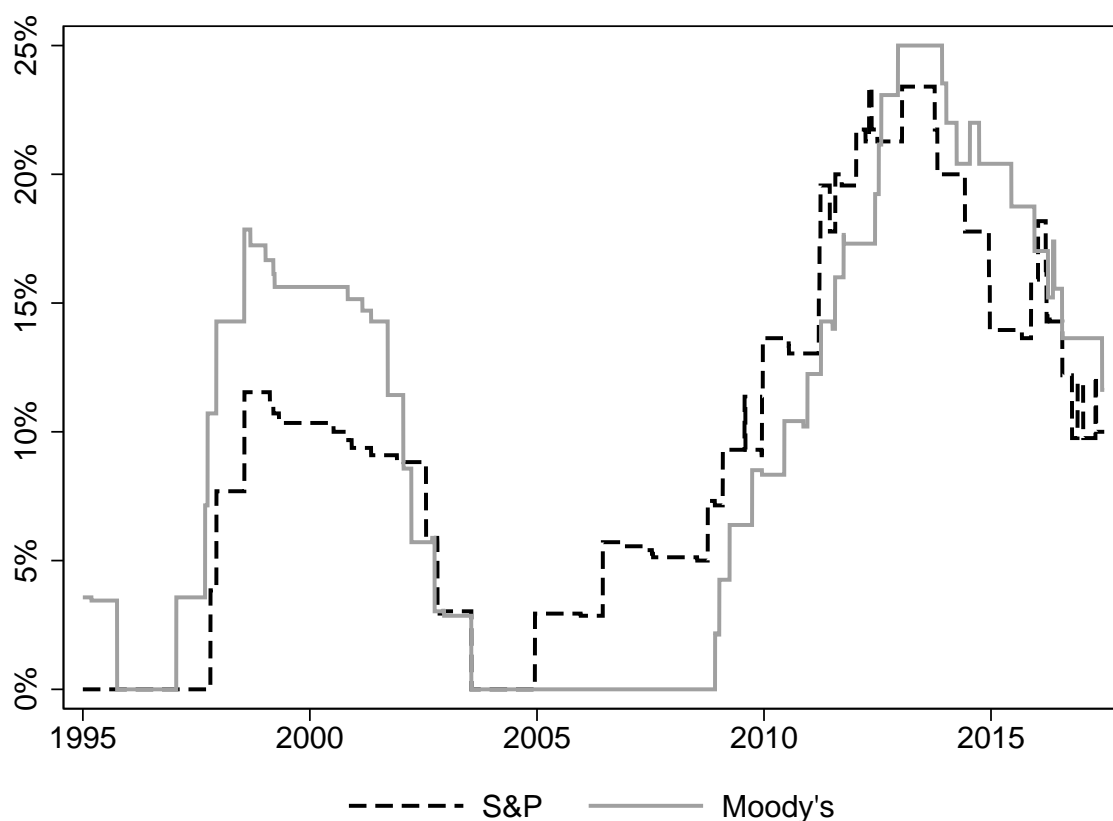
Figure 1: Probability of transitioning from A– or better to below A– over five years
